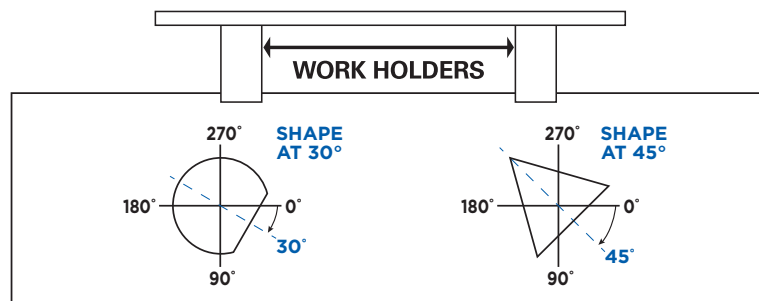
Front of Press — Punch View
