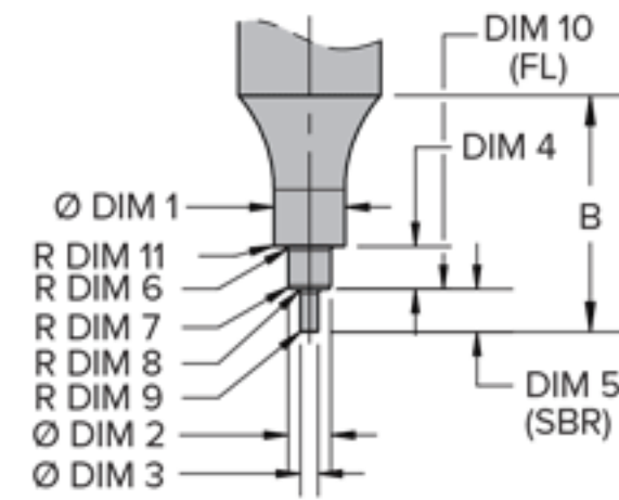
R06 CONE
