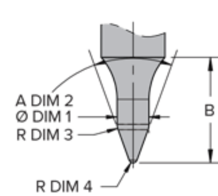
R06 CONE
