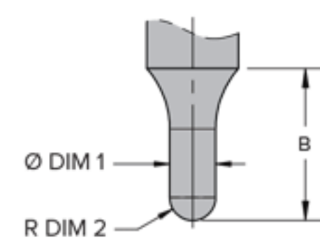
R11 SPHERICAL
