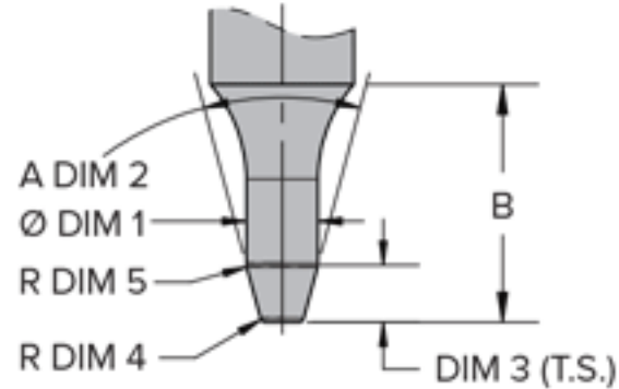
R12 EXTRUSION
