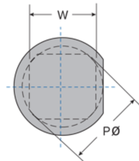
QD Quad-D
