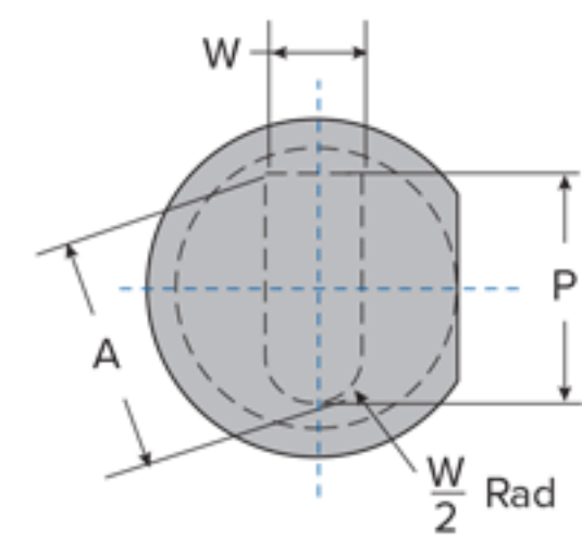
LD Long-D
