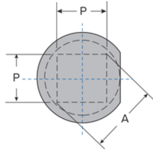
SQ Square
