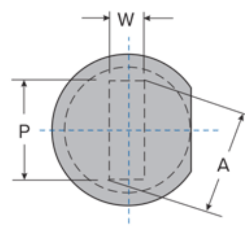
RT Rectangle
