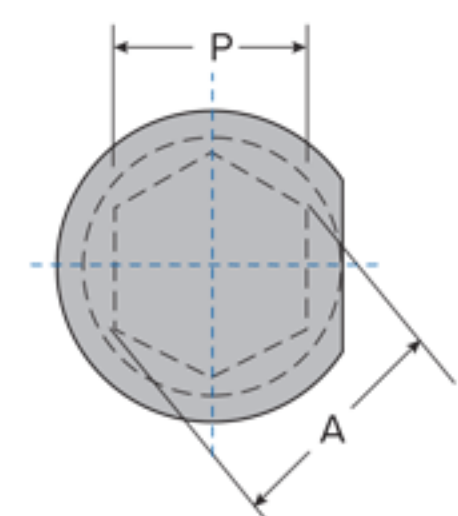
HX Hexagon
